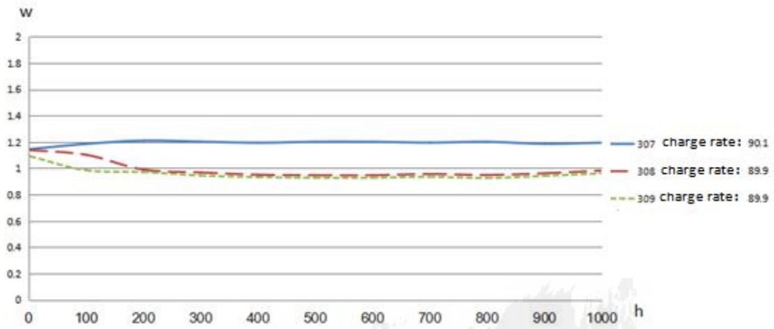
Fig 1 The Accelerated ageing curve of samples
