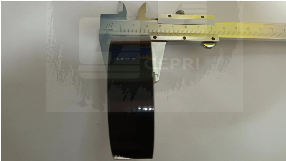
Fig D1: Outside view of MO resistor ( \Phi 78\text{mm} \times 23\text{mm} )
